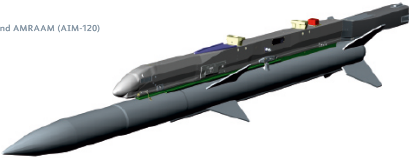
MML and SIDEWINDER (AIM-9)
