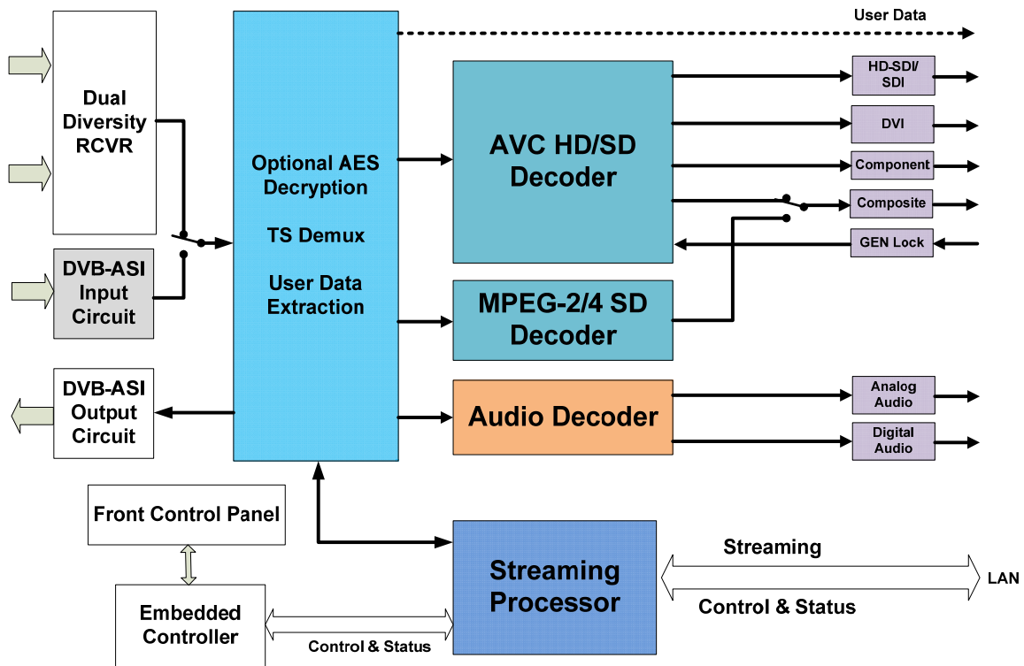
MVRD Block Diagram
