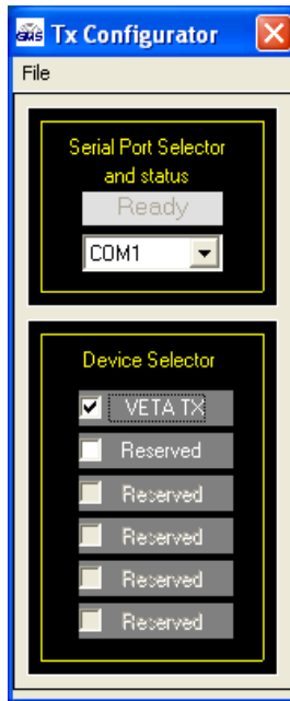
Figure 5.1 VETA Configurator
