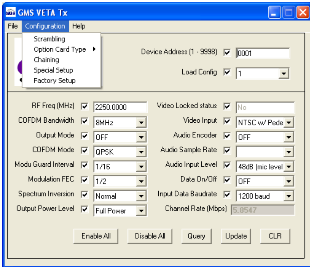
Figure 5.5 Configuration Menu
